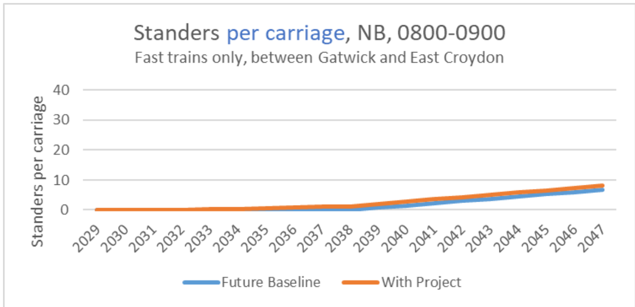
Diagram 9.6.14: Standers per carriage between Gatwick Airport and East Croydon
