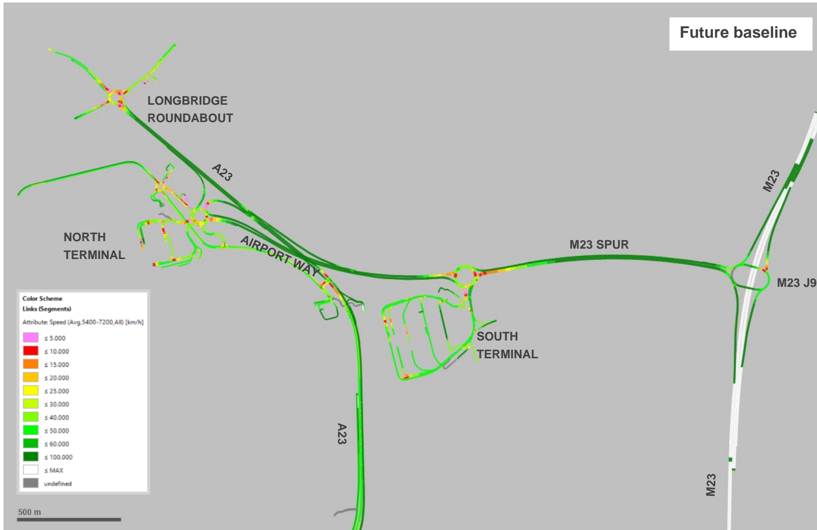
Diagram 13.5.9: 2032 future baseline– average speeds, PM peak 16:00-16:30
