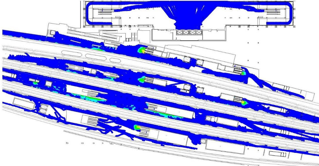
Diagram 10.8.11: Platform LoS, Fruin queuing – 2032 future baseline PM peak (17:00-17:15)
