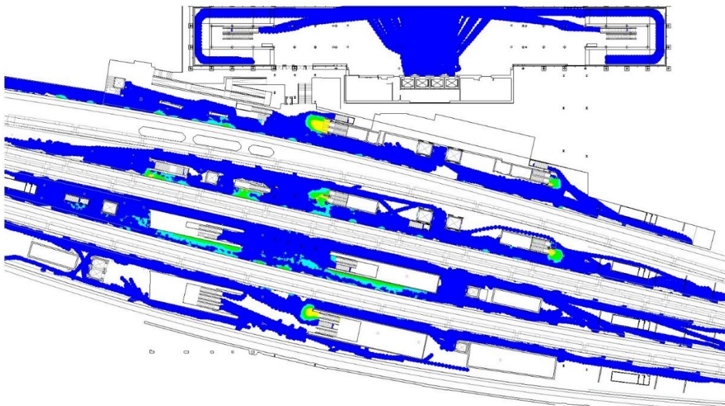
Diagram 10.8.12: Platform LoS, Fruin queuing – 2047 future baseline PM peak (17:00-17:15)
